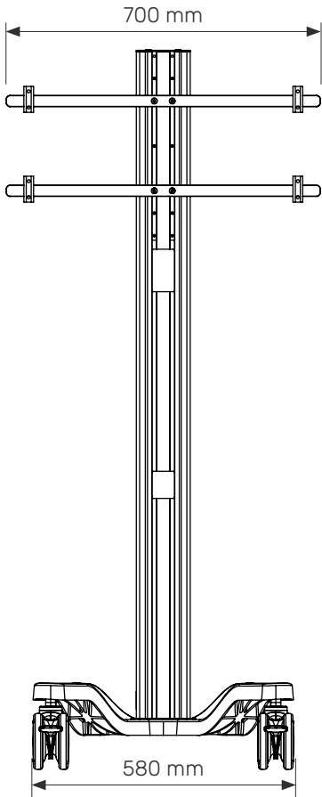
Front
